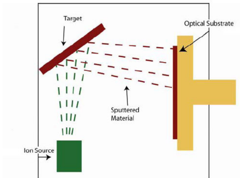
Fig. 4: The IBS process offers a high degree of control. Here an ion beam is used to sputter atoms off a target.
